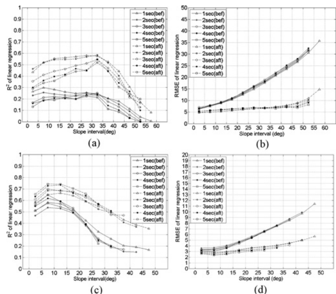
Fig. 5. Correlation between SRTM-NED and forest canopy height under different data resolutions and terrain slope intervals before and after the co-registration of SRTM and NED. (a) and (b) show the R^2 and RMSE for the CA site, respectively, whereas (c) and (d) show the R^2 and RMSE for the NH site, respectively.
