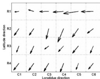
Fig. 3. Horizontal translation of SRTM relative to NED. The length of the arrows represents relative magnitude of the displacement
