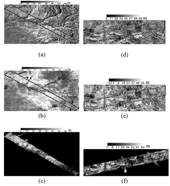
Fig. 2. Differences between SRTM and NED before and after the co-registration of SRTM and NED. (a) Difference between original SRTM and NED at CA. (b) Difference between registered SRTM and NED at CA. (c) RH100 from LVIS data at CA. (d) Difference between original SRTM and NED at NH. (e) Difference between registered SRTM and NED at NH. (f) RH100 from LVIS data at NH. The polygons in (a), (b), (d), and (e) are the area covered by LVIS data
