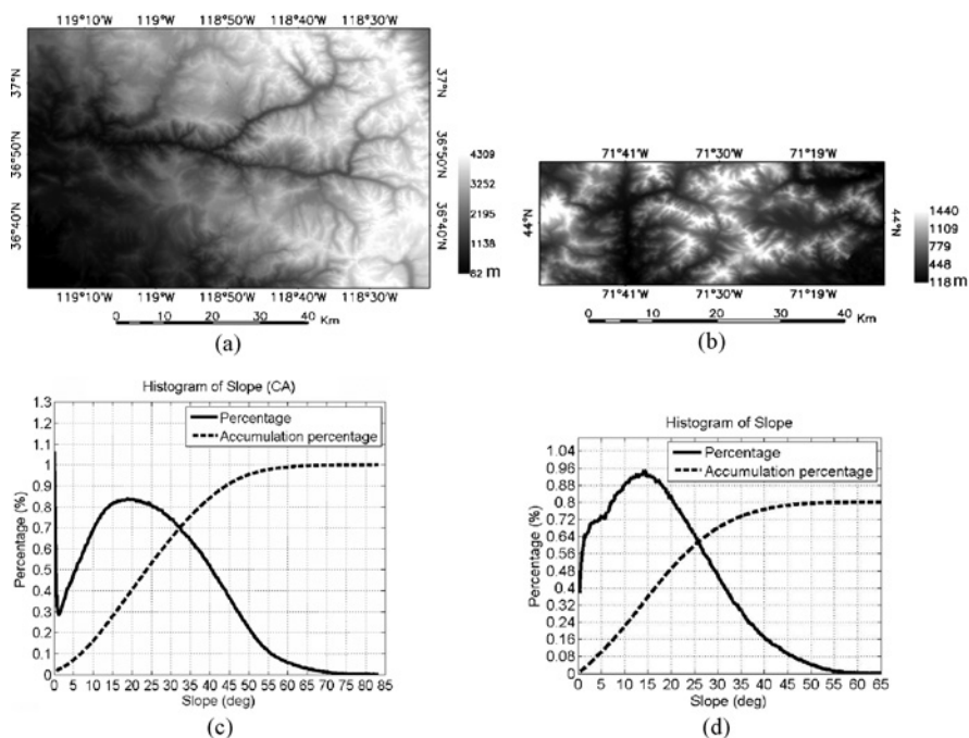
Fig. 1. Location and terrain conditions of the California (CA) and New Hampshire (NH) test sites. (a) NED of the California site. (b) NED of the New Hampshire site. (c) Histogram of the terrain slope of (a). (d) Histogram of the terrain slope of (b). The vertical grid is 10% for the accumulation percentage in (c) and (d).
