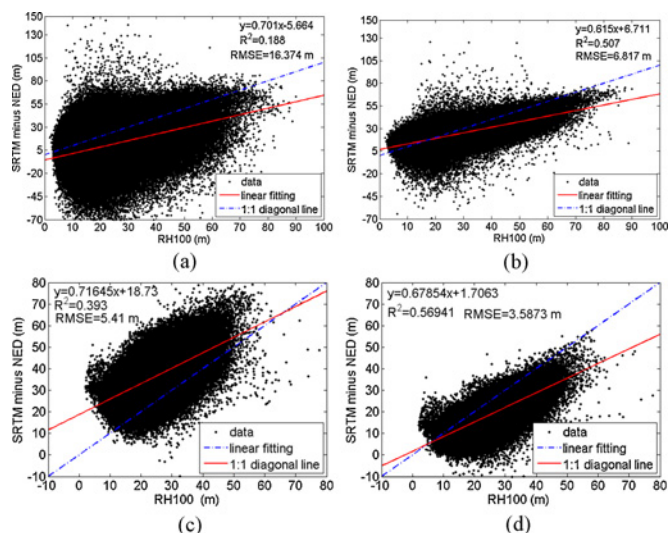
Fig. 4. Scatter plots of SRTM-NED versus RH100 (a) before registration (CA site), (b) after registration (CA site), (c) before registration (NH site), and (d) after registration (NH site).
